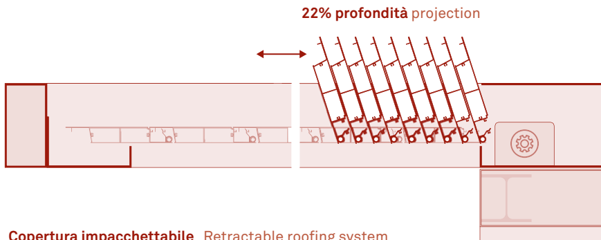
FOLD 220 Copertura impacchettabile Retractable roofing system
